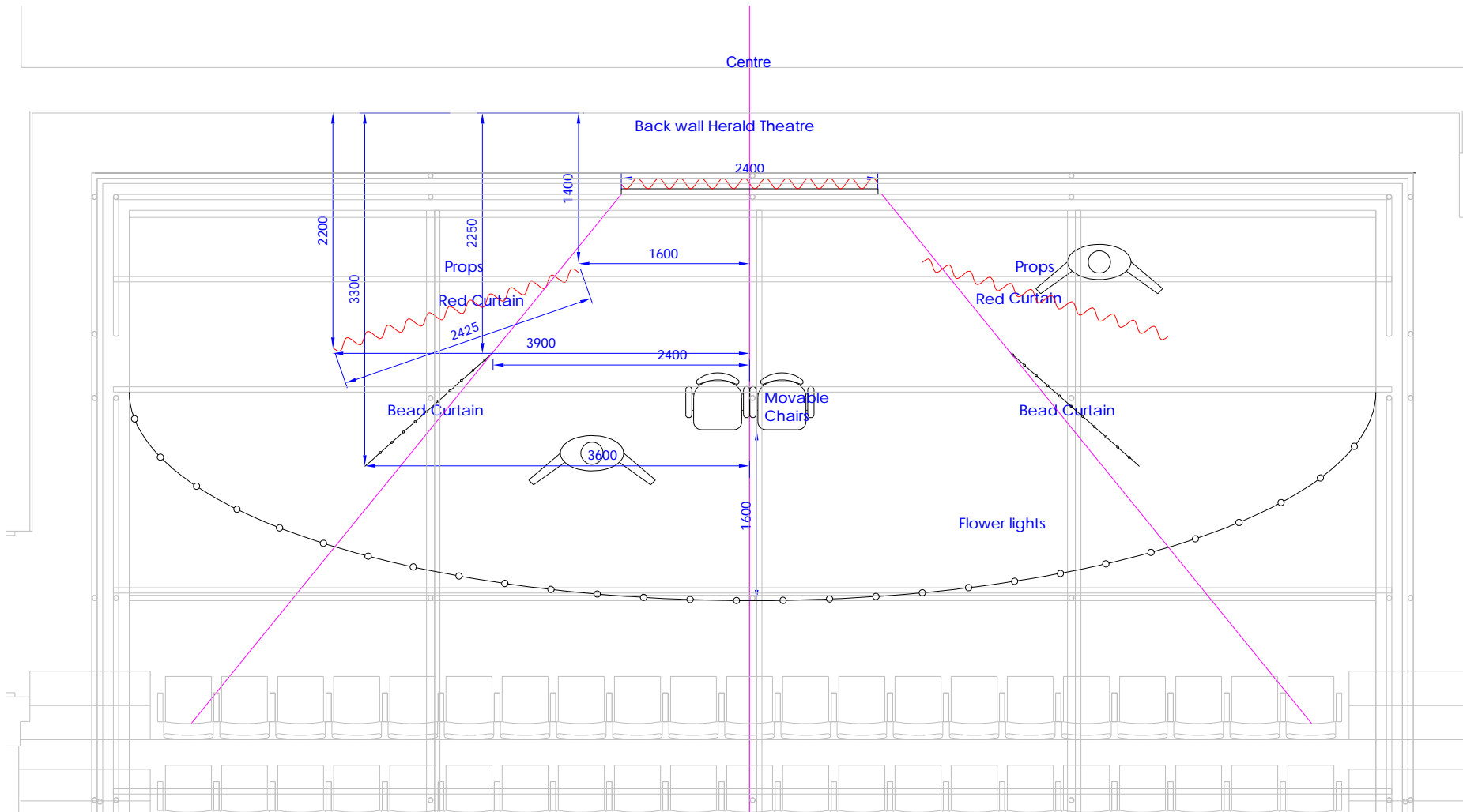
FROM INDIA WITH LOVE floor plan
